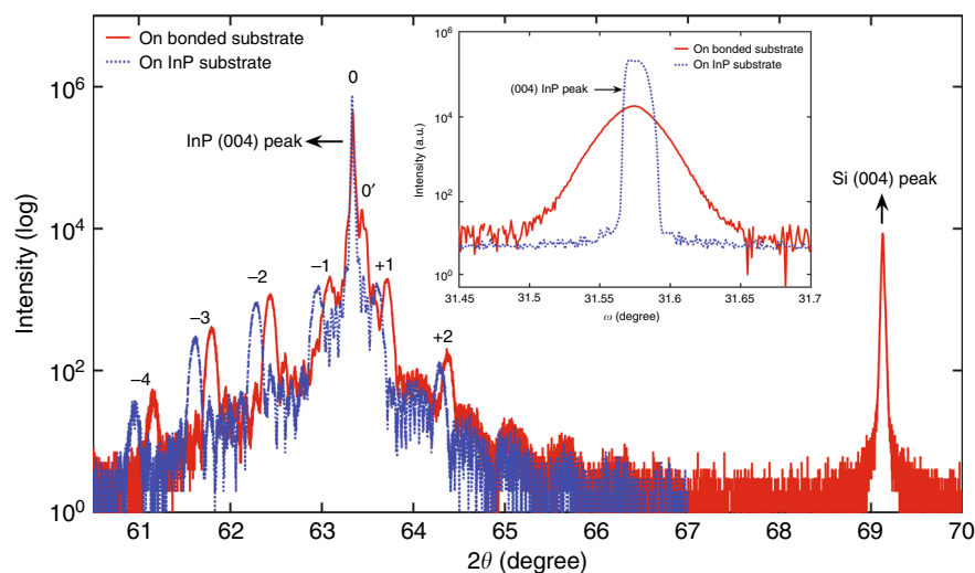
Fig. 3 High-resolution XRD \omega - 2\theta measurements of the epitaxy. Inset: high-resolution omega scans of the InP (004) peak
