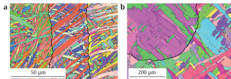
Fig. 10 Effect of heat treatment temperature on microstructure. a EBSD orientation map of post-process heat treated at sub-transus 850°C/2h/FC 84 . b EBSD orientation map of post-process heat treated at super-transus 1020°C/0.5h followed by sub-transus 730°C/2h/AC 84 . The deposition direction in both images is in vertical direction.
