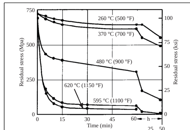
Fig. 9 Effect of stress-relieving temperatures on residual stress in Ti-6Al-4V 3 .
