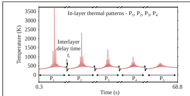
Fig. 4 Simulated thermal cycling history of a specific location in LPBF fabricated Ti-6Al-4V. This includes intralayer and interlayer reheating and cooling. P1 to P5 are different layers 40 .
