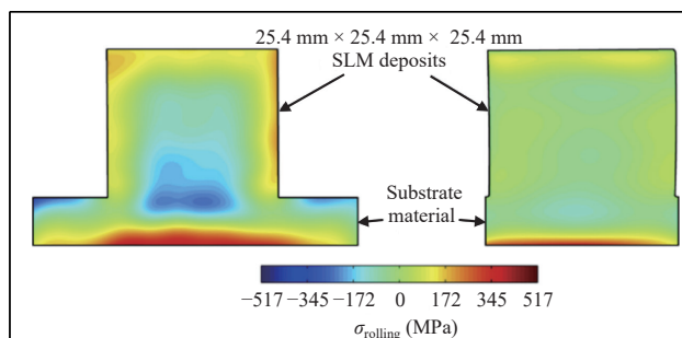
Fig. 5 Residual stress of LPBF fabricated Ti-6Al-4V measured via contour-method in the rolling direction of the substrate. Specimens are built on a large substrate with an overhang (left) and a small substrate without an overhang (right) 50 .
