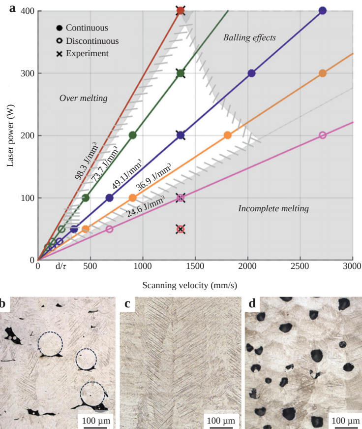
Fig. 3 A process window and various types of defects in LPBF fabricated Ti-6Al-4V. a A processing window for LPBF fabricated Ti-6Al-4V 38 . b–d The influence of scan speed on porosity types in LPBF fabricated Ti-6Al-4V with a fixed laser power of 175 W and a hatch distance of 100 μm 36 . b Lack-of-fusion due to insufficient penetration at a high scan speed. c A nearly fully dense microstructure density at an intermediate scan speed. d Keyhole type defects due to overheating at a low scan speed.
