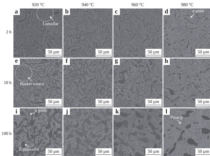
Fig. 11 Effect of sub-transus solution temperature and time on microstructure. SEM images of LPBF fabricated Ti-6Al-4V after different \alpha+\beta STA heat treatments. The results show the effect of solution temperature and time on the microstructure evolution; all the solution treatments are followed by AC and a subsequent aging treatment at 700 °C/2 h/FC 105 .
