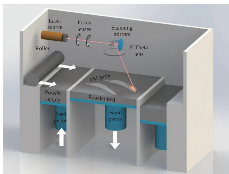
Fig. 2 Schematic diagram of a typical LPBF system 24 .
