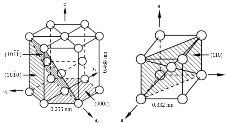
Fig. 1 Crystal structures of HCP \alpha and BCC \beta phases in titanium 1 .
