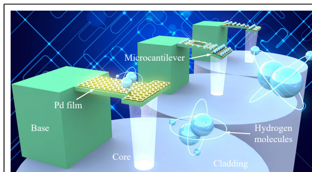
Fig. 1 Schematic of rectangular solid, rectangular hollow, and triangular polymer microcantilever probes for hydrogen sensing on an optical fiber tip.
