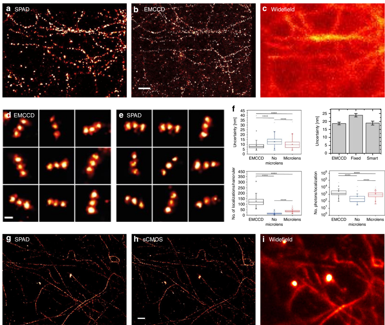
Fig. 5 SPAD super-resolution images. a The first super-resolution image captured with SwissSPAD, compared to b EMCCD and c widefield images. The images show the microtubuli of an U2OS cell labelled with Alexa Fluor 647, in Vectashield 129 . d, e Comparison of the SPICImager using “smart” aggregation and microlenses with an EMCCD. The images show multiple GATTA-PAINT 40G nanoruler localisations 45 . f Comparison of the differences in localisation uncertainty with and without “smart” aggregation and the impact of the microlenses 45,130 . g SwissSPAD super-resolution image of microtubuli labelled with Alexa 647 in OxEA buffer compared to h sCMOS and i widefield images 129 . The white bar indicates 1 \mu m. The images are reprinted from refs. 45,129,130
