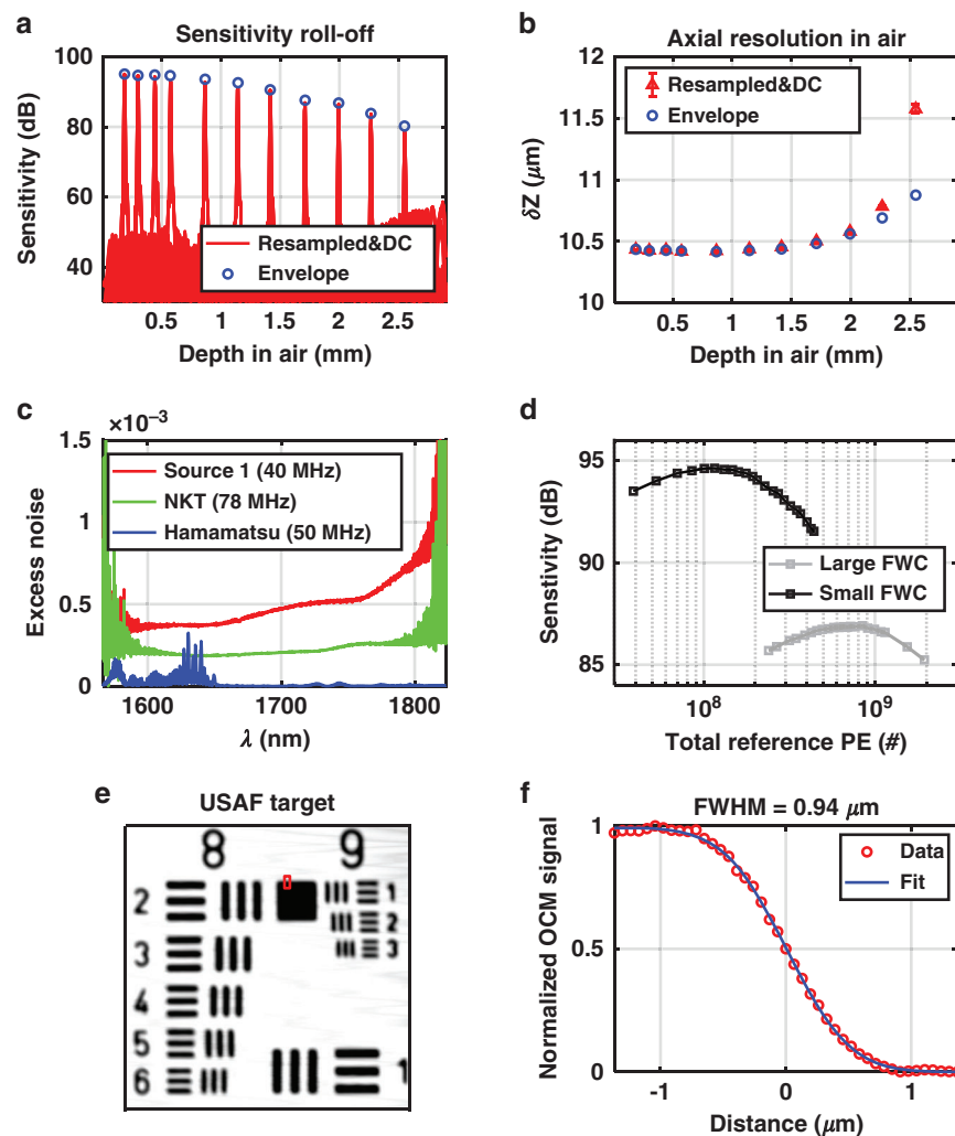
Fig. 8 1700 nm OCM system characterization. a Sensitivity roll-off and b axial resolution versus depth. To assess efficacy of resampling and dispersion compensation (DC), results (red) are compared with theoretical values from the envelope (blue circles). c Excess noise coefficient measurements of three light sources. d System sensitivity using Hamamatsu light source with large ( 12.5 \text{ Me}^- ) or small ( 1.25 \text{ Me}^- ) full well capacity (FWC) camera settings. e En face image of groups 8 and 9 of a negative USAF 1951 target. f Measured edge response (red circles), from the red box in e , are fitted with an error function (blue line) to yield the transverse resolution
